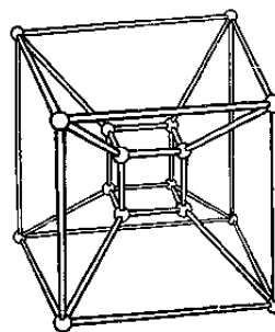
5. Perspective representation of a four-dimensional cubic lattice seen in four-space.
