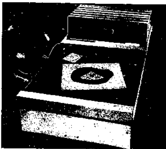
17. The “Numa-Rete”, an artificial “retina” counting the number of objects independent of their size, location and form, and independent of strength of illumination.
