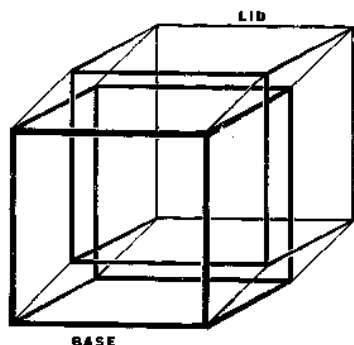
4. Three-dimensional lattice of an obliquely projected four-dimensional cube parallel to our three-space.
